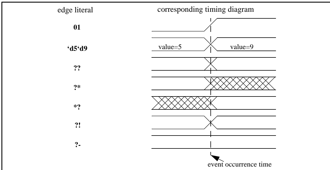
Figure 17—Timing diagram for single events
