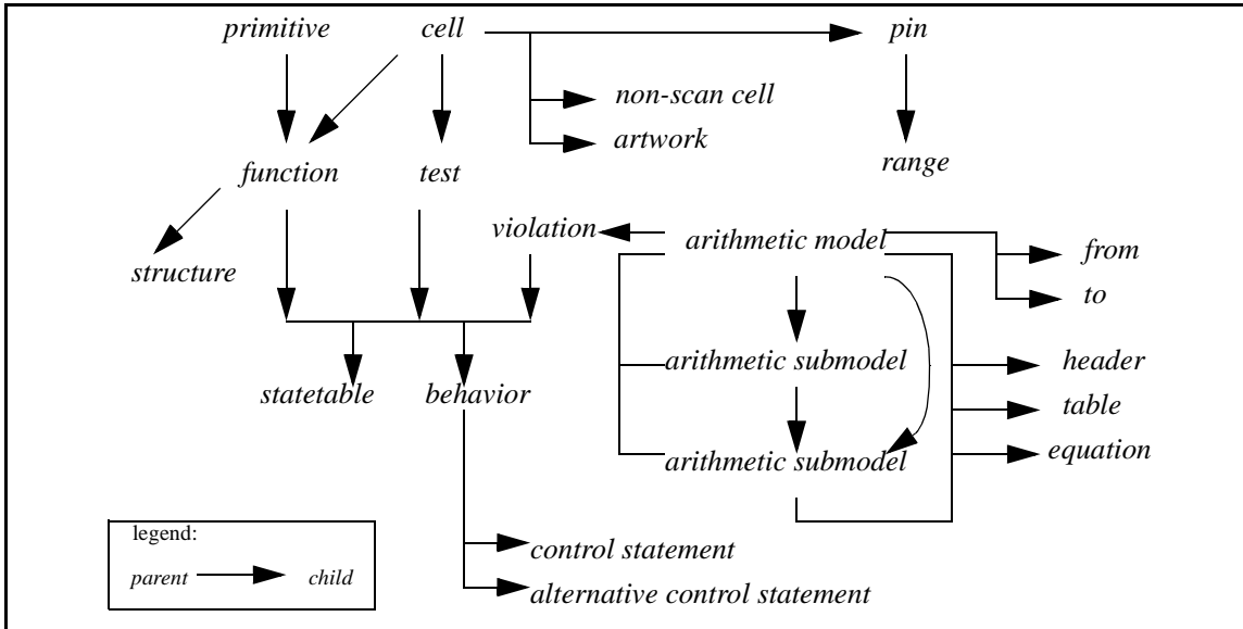
Figure 7—Parent/child relationship involving singular statements and plural statements
