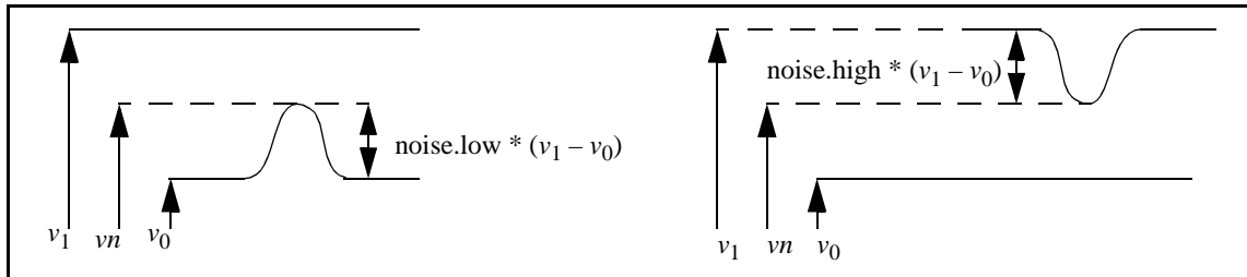
Figure 35—NOISE measurement definition
