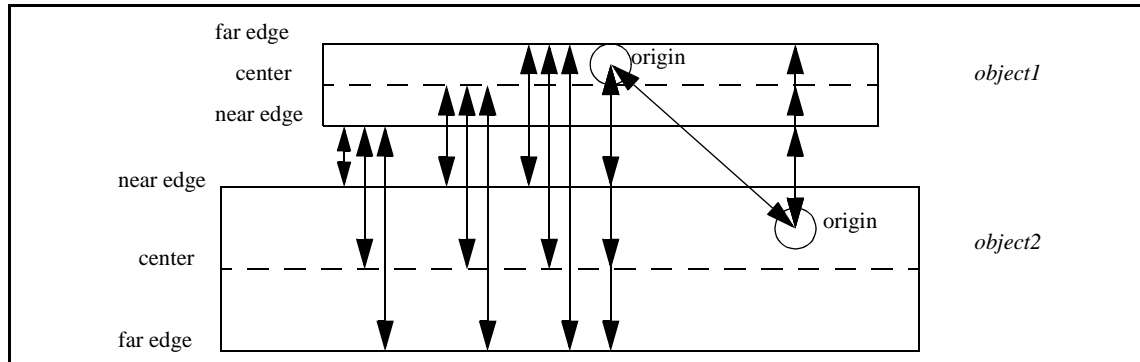
Figure 46—Illustration of REFERENCE for DISTANCE
