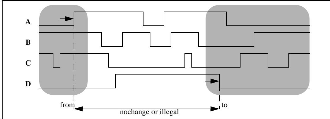
Figure 29—Illustration of NOCHANGE and ILLEGAL
