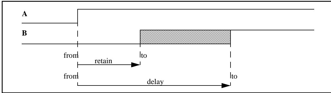
Figure 25—Illustration of RETAIN and DELAY
